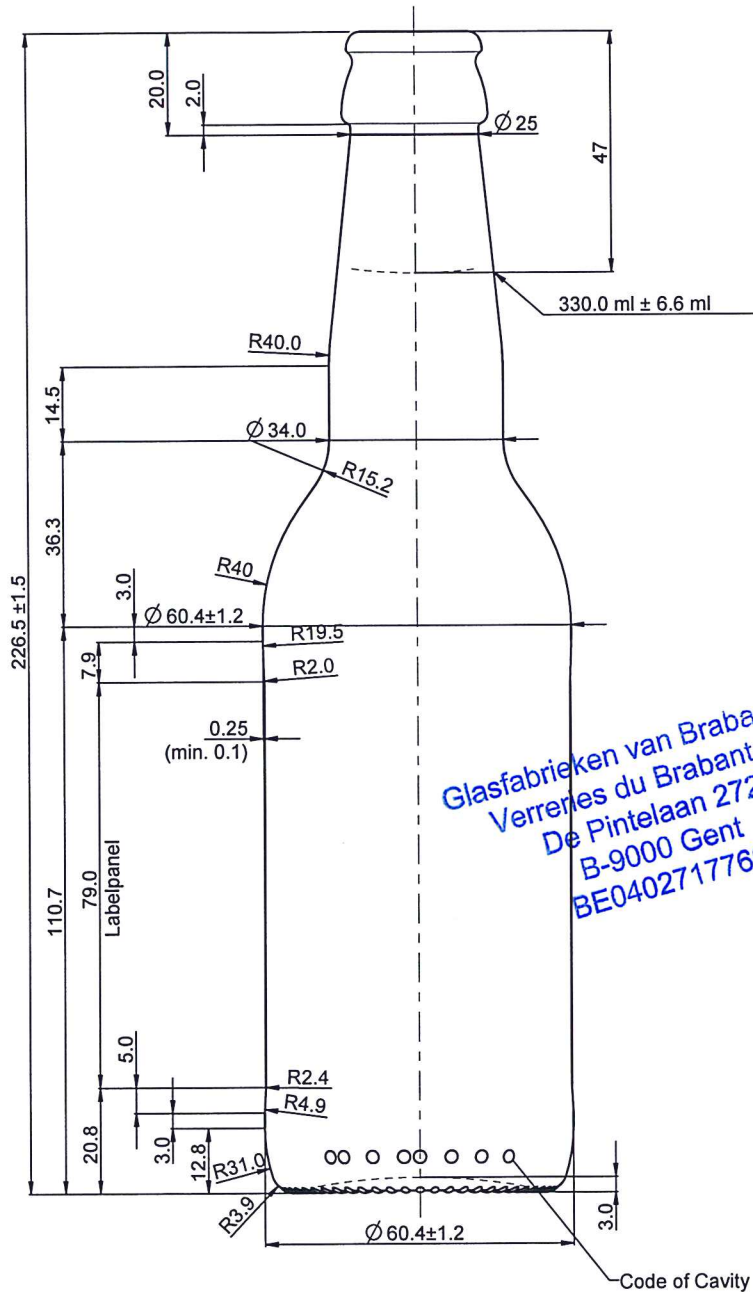
Front view 26H 180 Crown Cork CE.T.I.E. GME 13.01:2007-06
